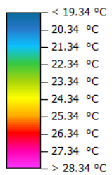
Potential Air Temperature
