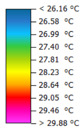
Potential Air Temperature
